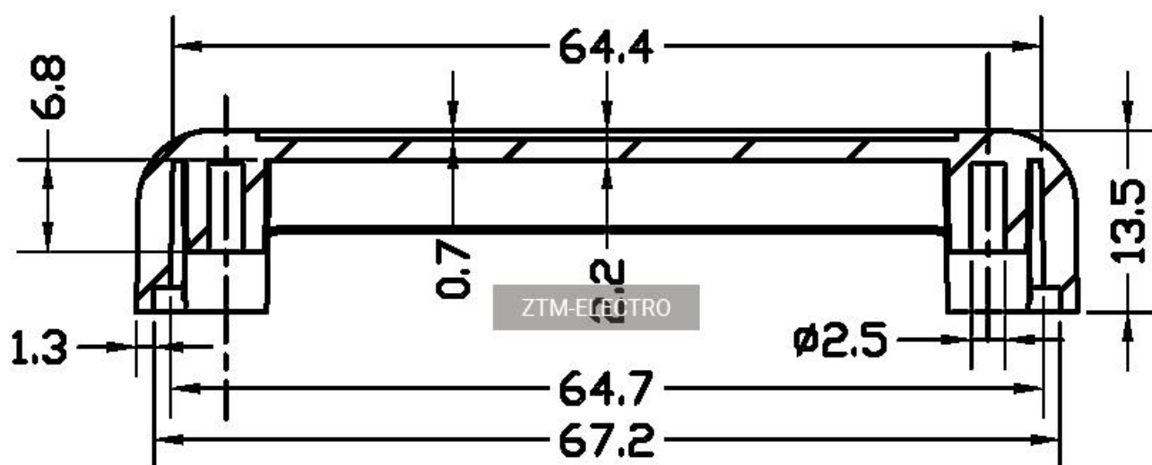
SECTION C—C
